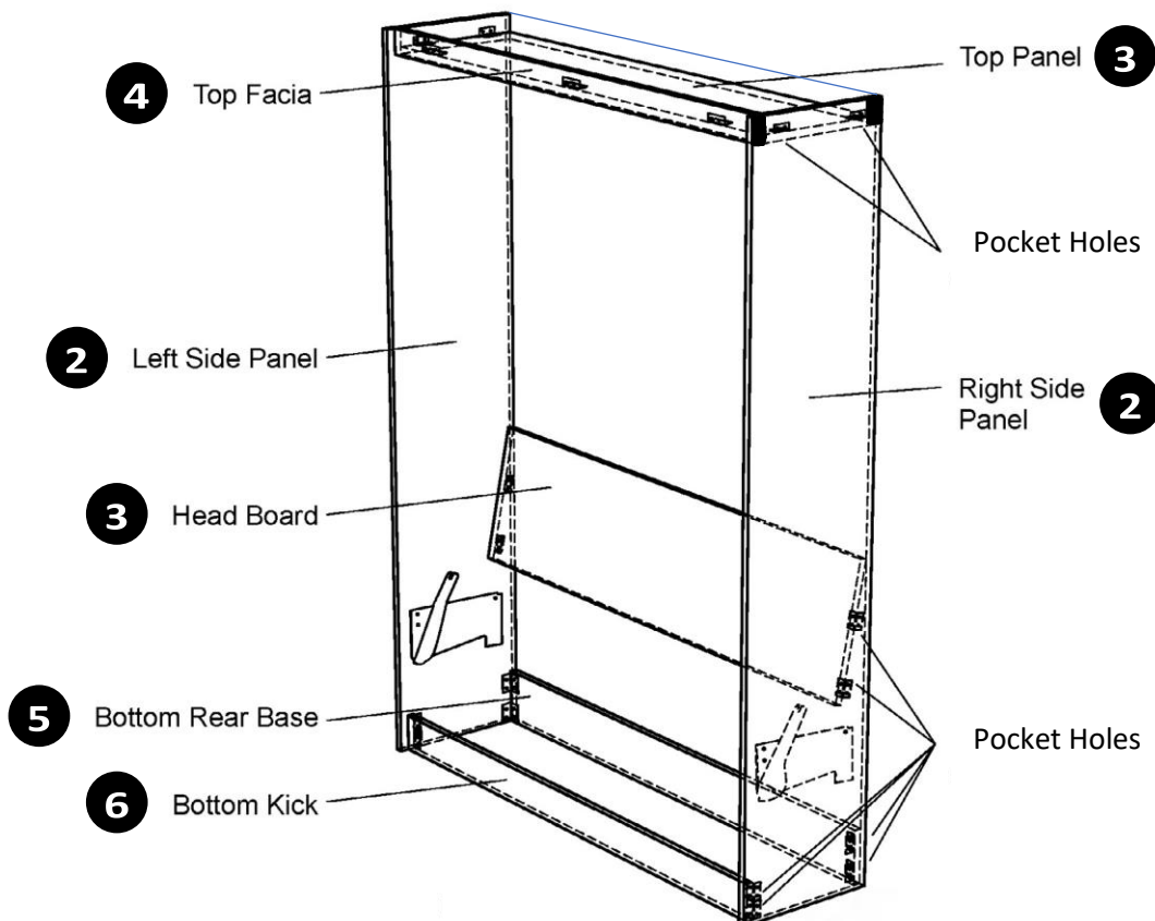
Drawing 3.
