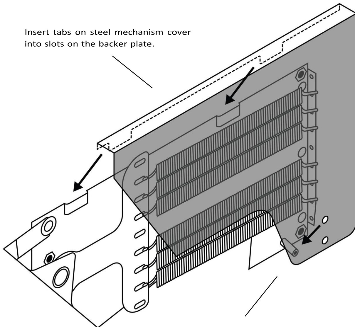
DRAWING 16.
