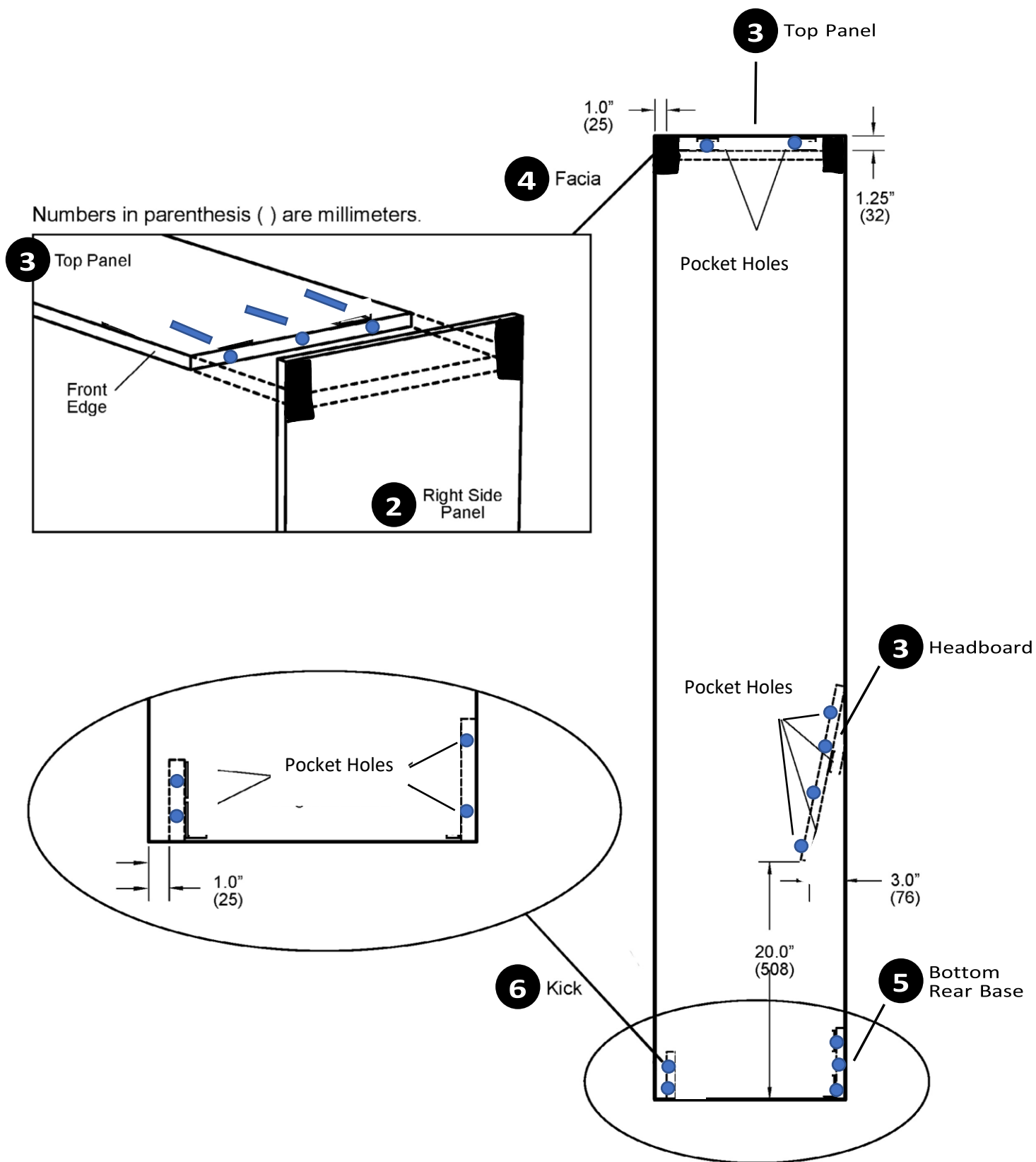
Drawing 4.
