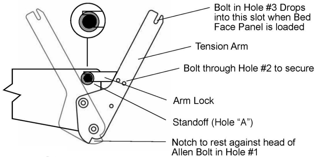
DRAWING 11.
