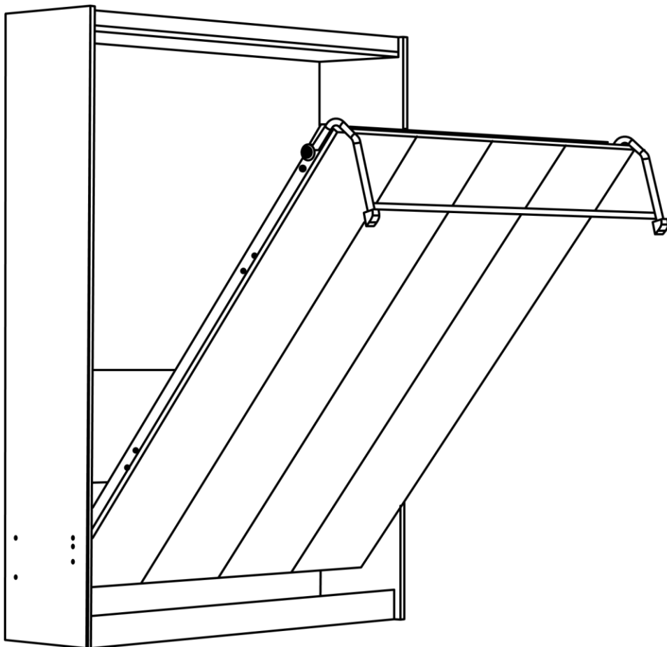
DRAWING 17.
