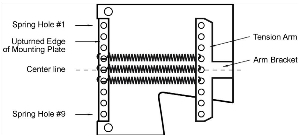
DRAWING 2.
